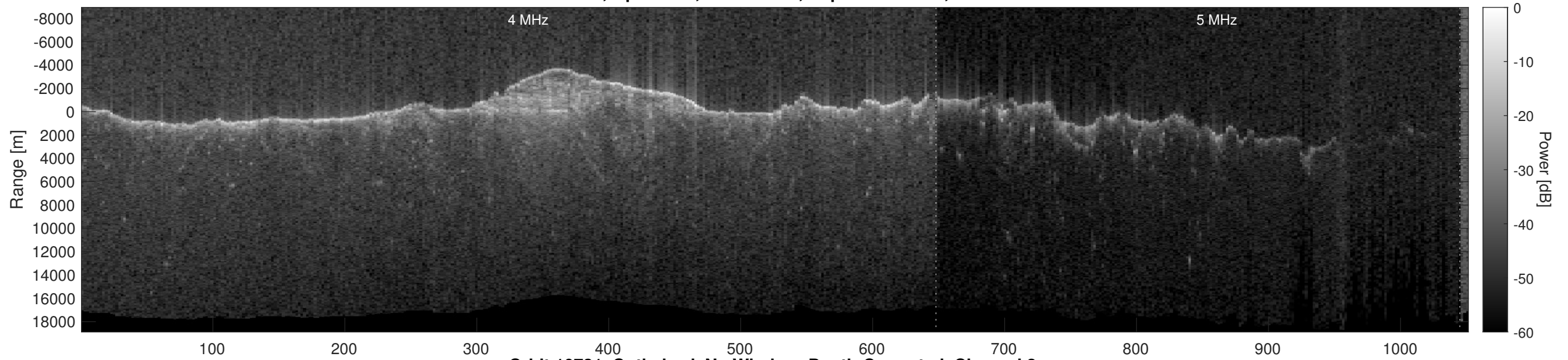
Orbit 10731, Optimized, No Window, Depth-Corrected, Channel 2
