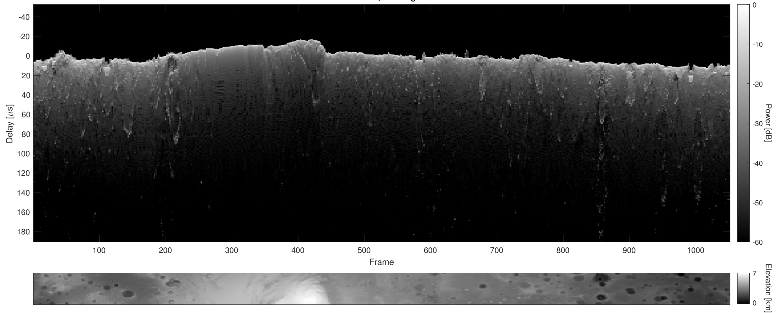
Orbit 10732, Cluttergram
