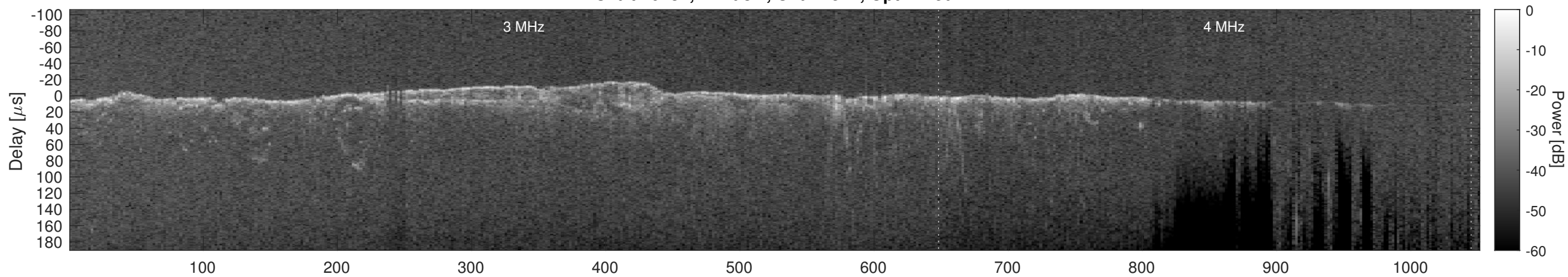
Orbit 10732, Cluttergram
