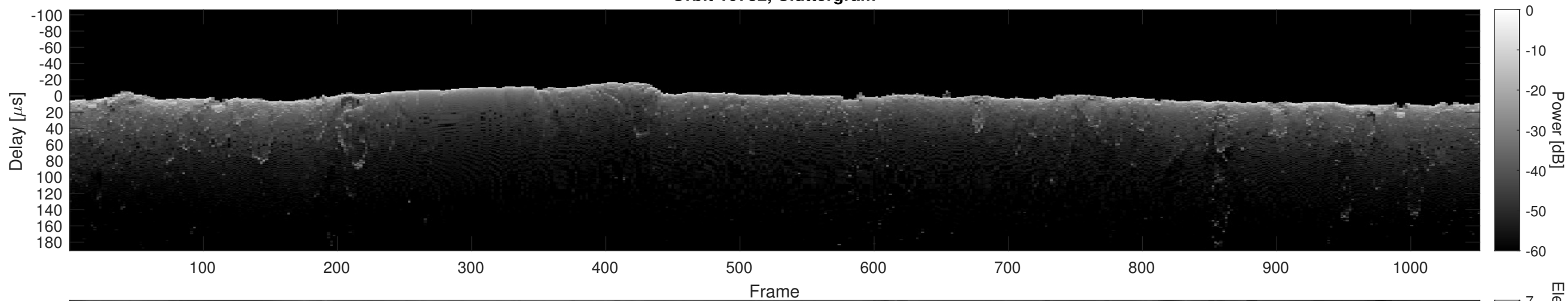
Orbit 10732, Cluttergram
