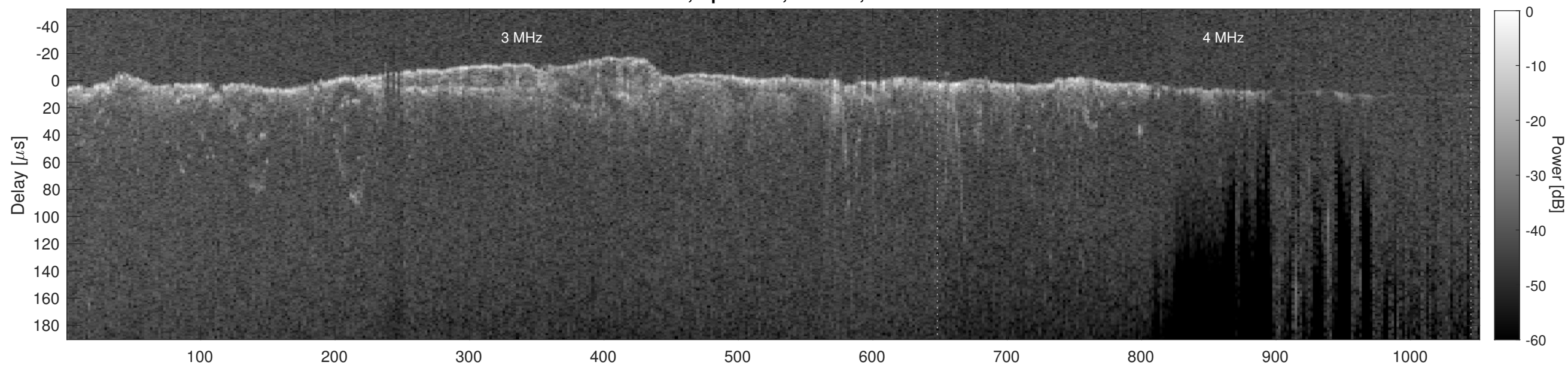
Orbit 10732, Cluttergram
