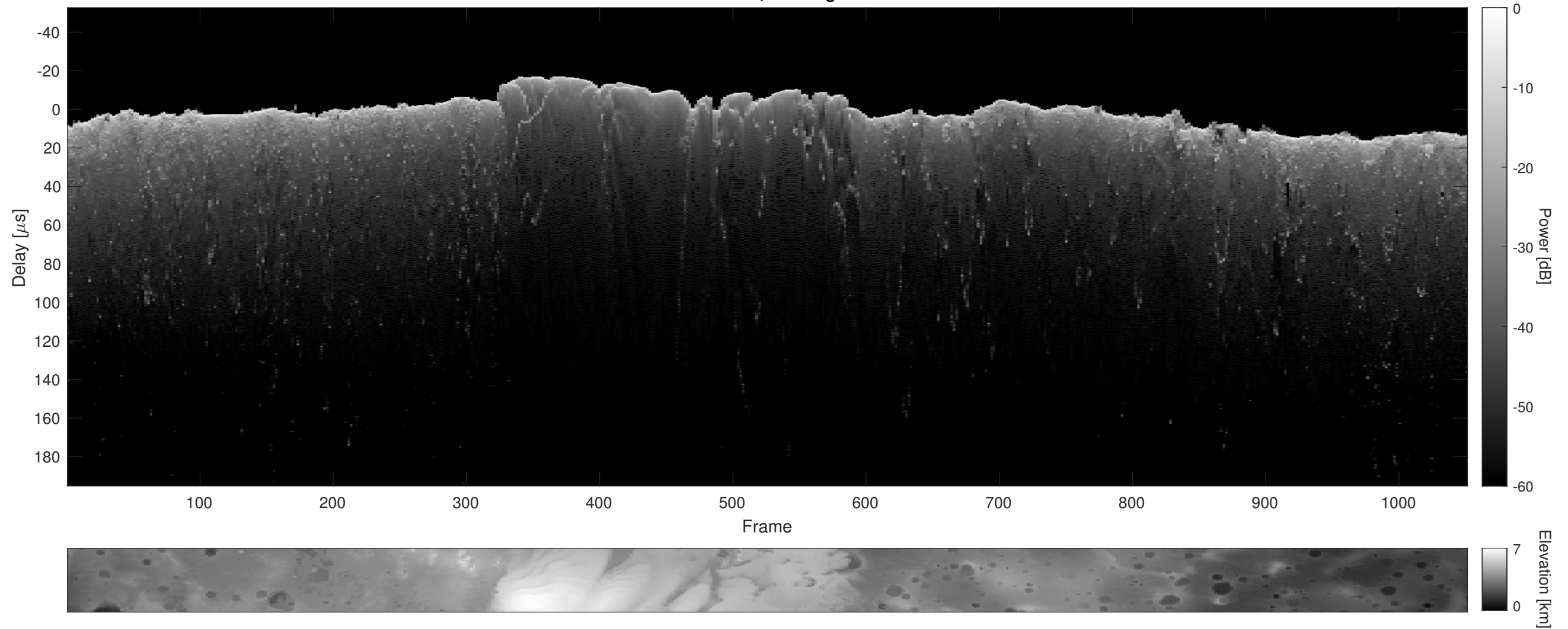
Orbit 10734, Cluttergram
