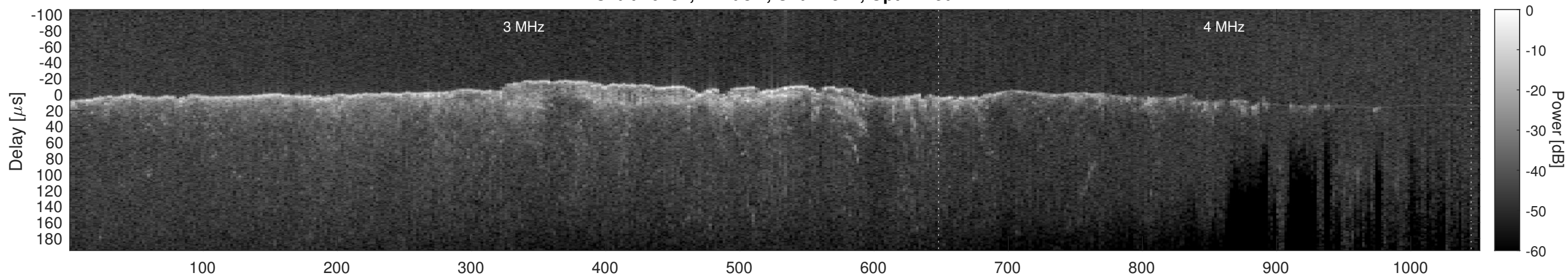
Orbit 10734, Cluttergram
