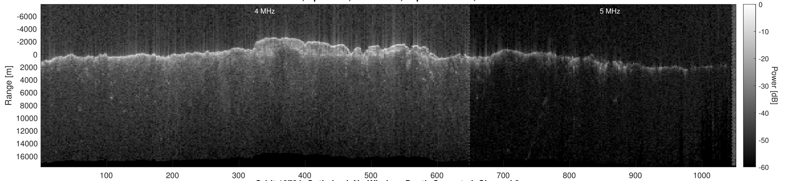
Orbit 10734, Optimized, No Window, Depth-Corrected, Channel 2
