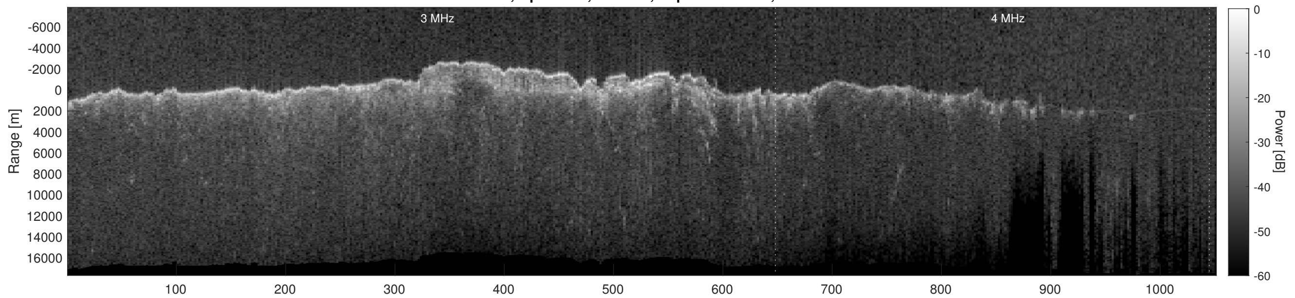
Orbit 10734, Depth-Corrected Cluttergram
