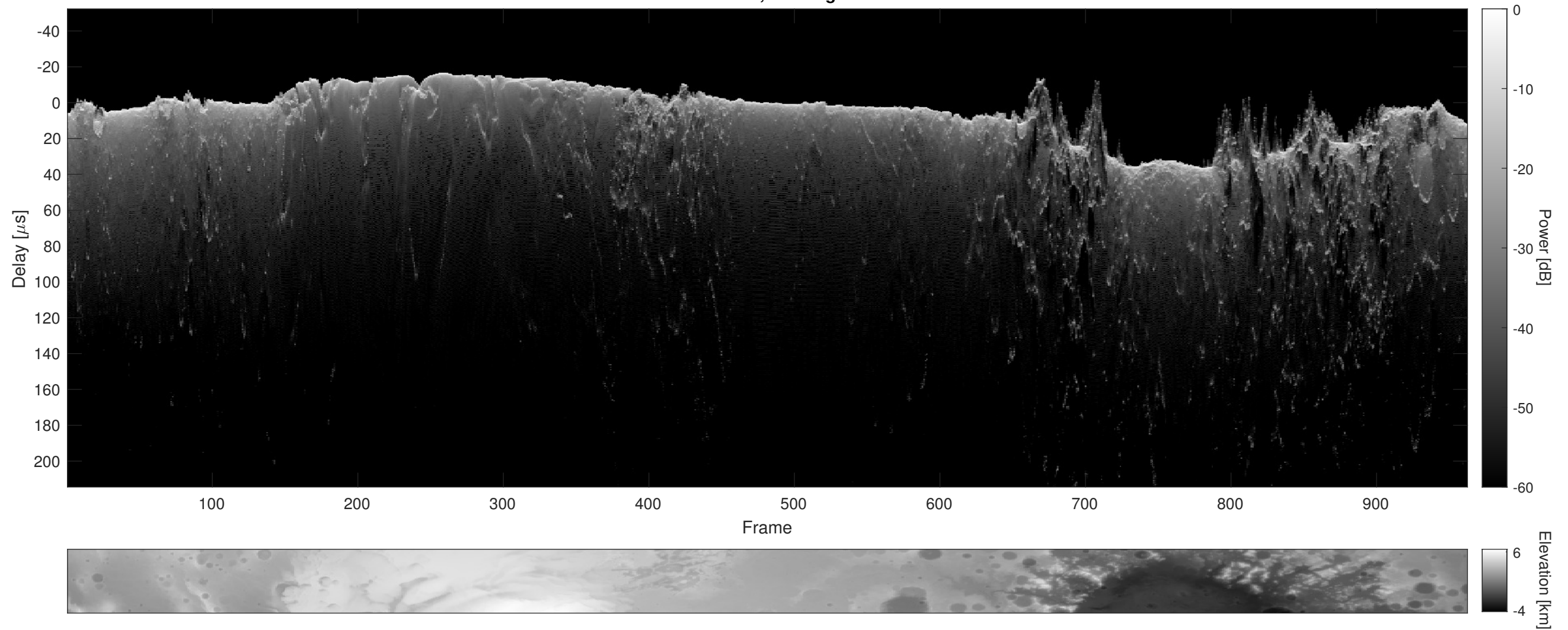
Orbit 10736, Cluttergram
