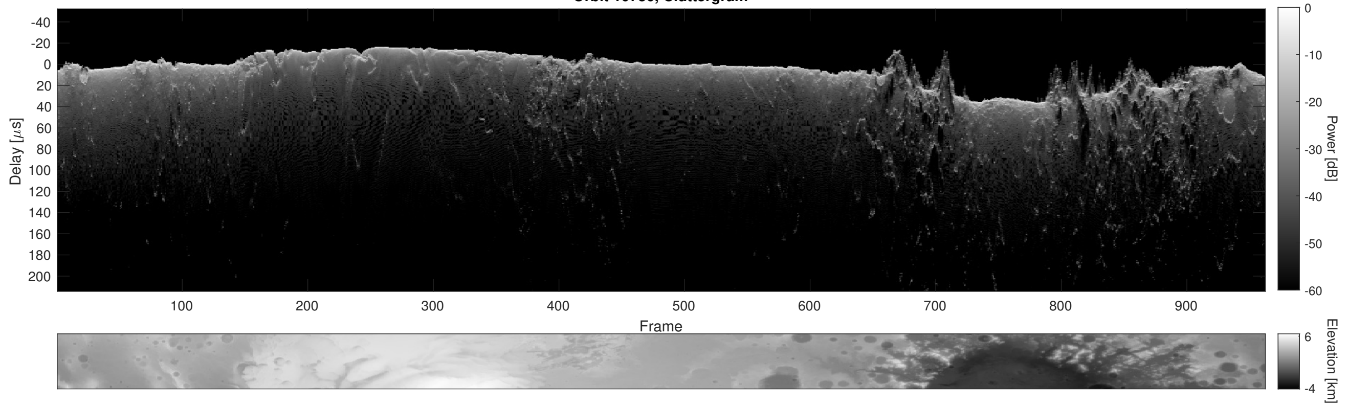
Orbit 10736, Cluttergram
