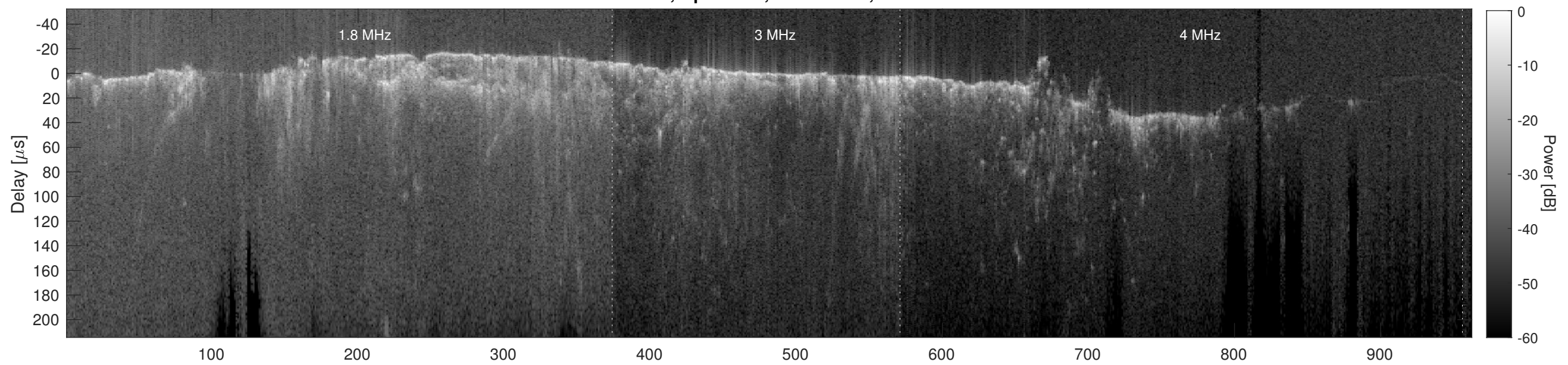
Orbit 10736, Cluttergram
