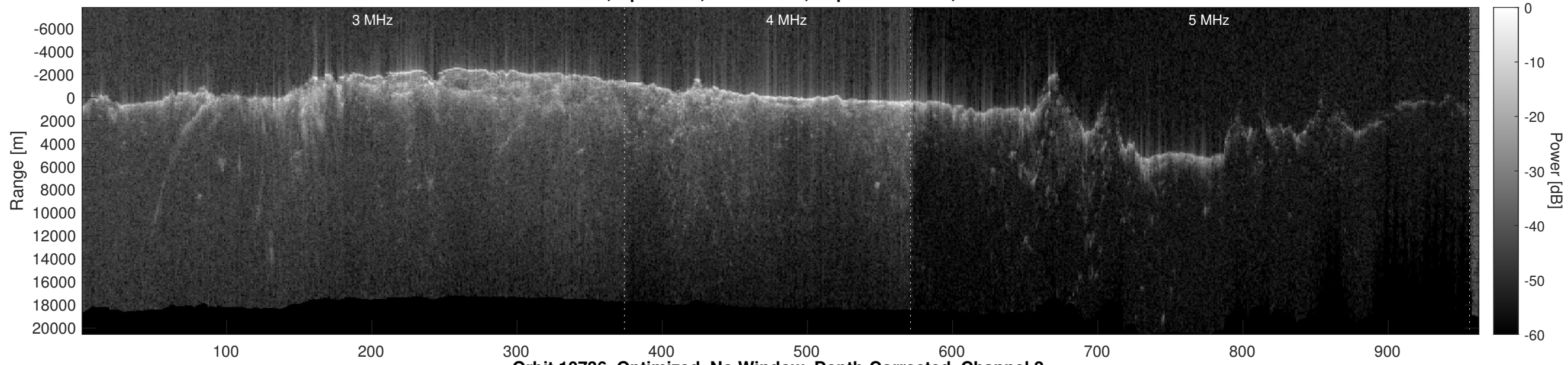
Orbit 10736, Optimized, No Window, Depth-Corrected, Channel 2
