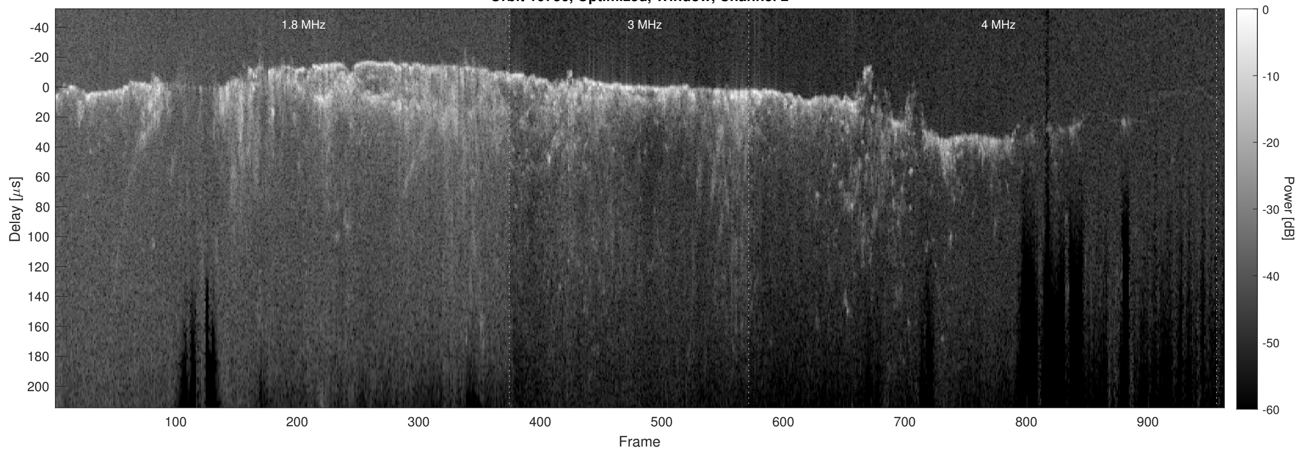
Orbit 10736, Optimized, Window, Channel 2
