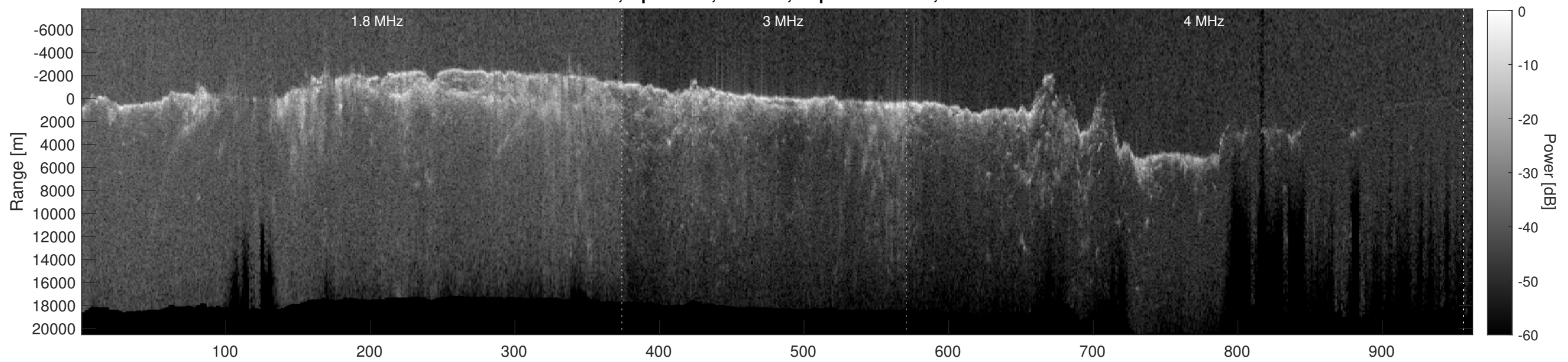
Orbit 10736, Depth-Corrected Cluttergram
