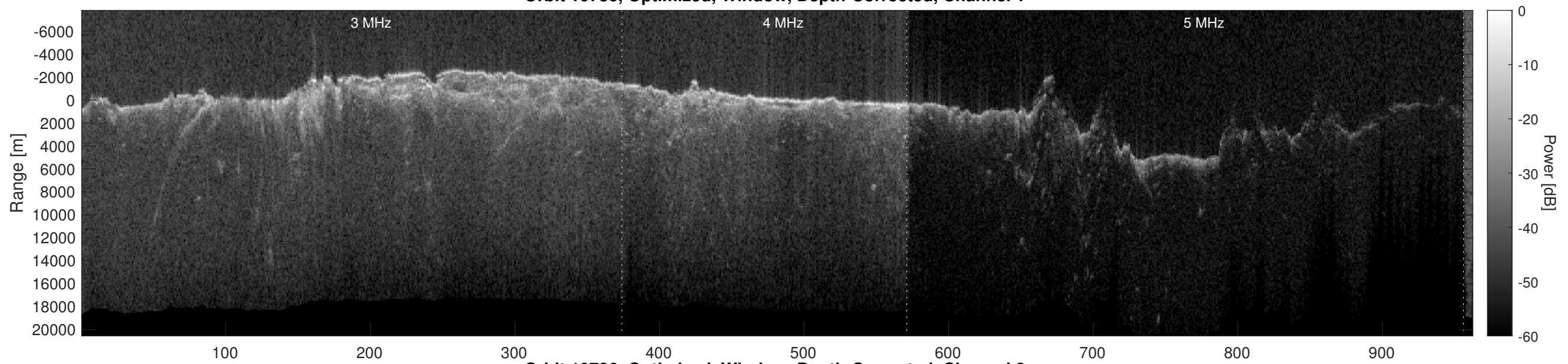
Orbit 10736, Optimized, Window, Depth-Corrected, Channel 2
