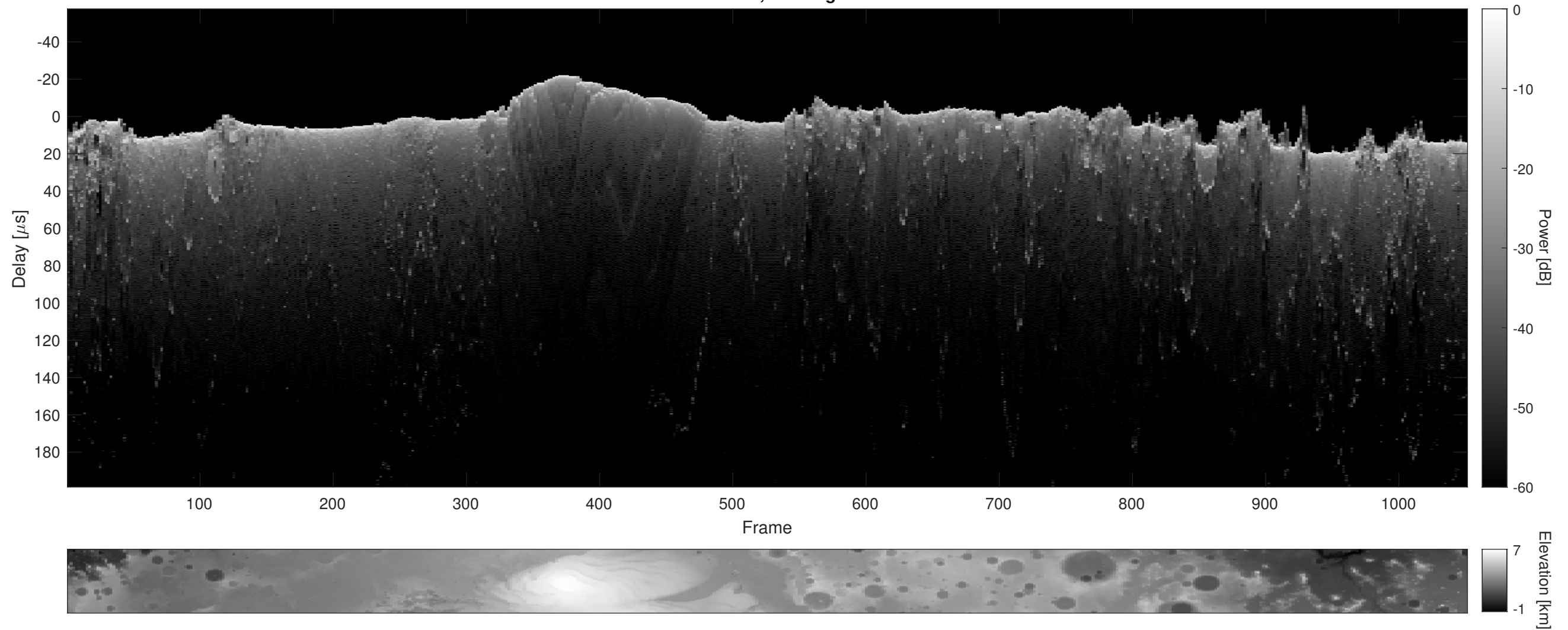
Orbit 10738, Cluttergram
