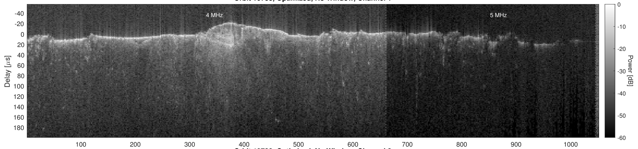
Orbit 10738, Optimized, No Window, Channel 2
