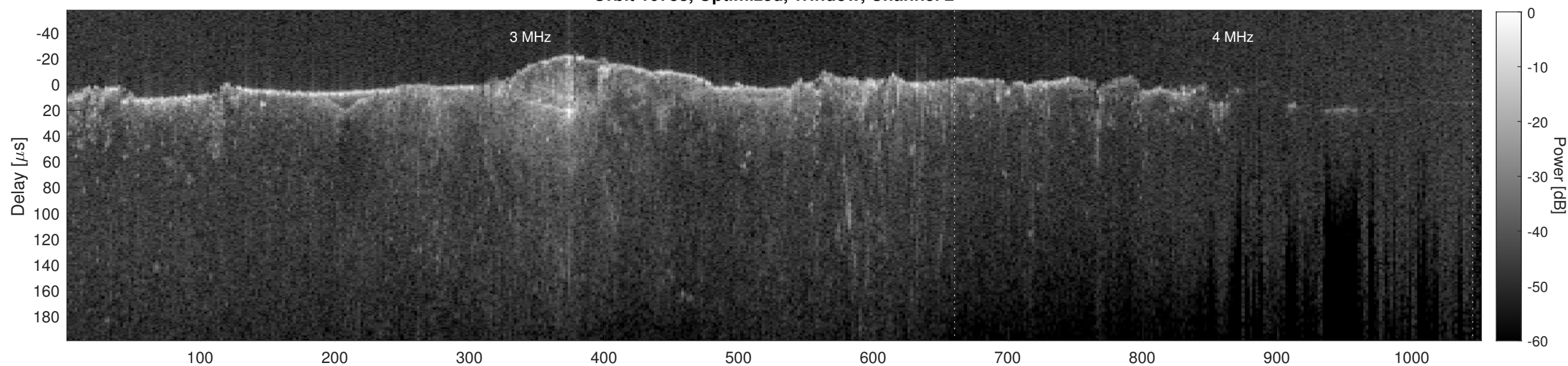
Orbit 10738, Cluttergram
