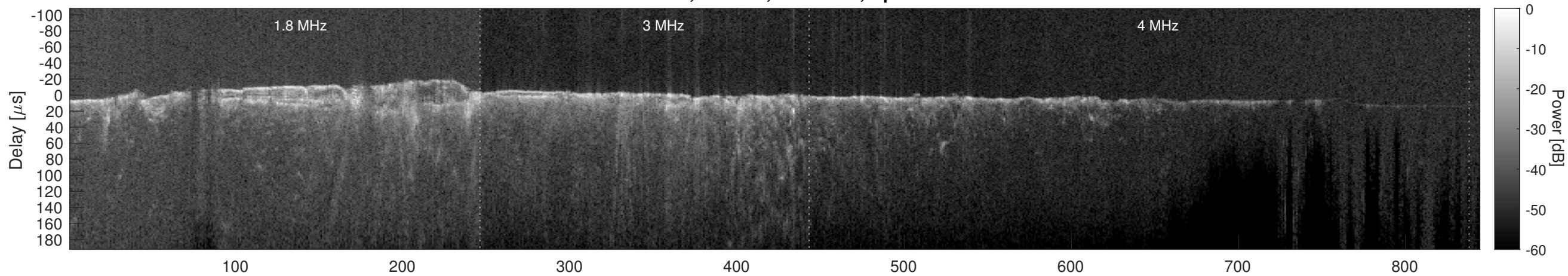
Orbit 10739, Cluttergram
