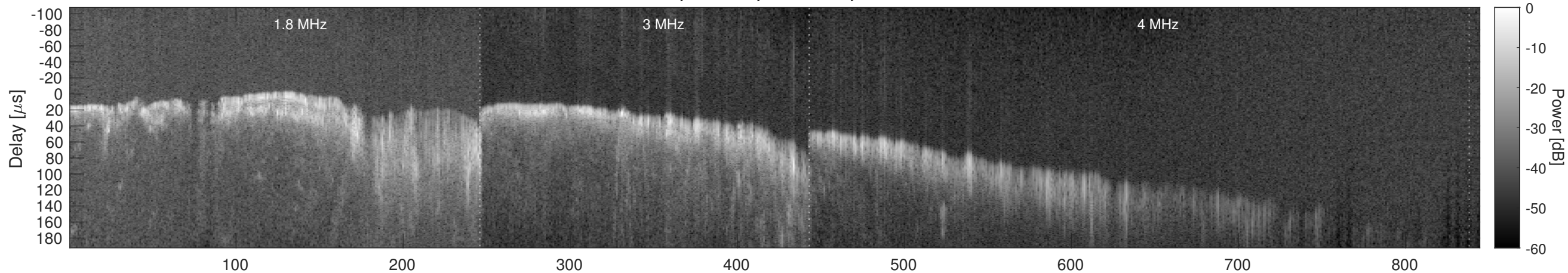
Orbit 10739, Window, Channel 2, Chapman
