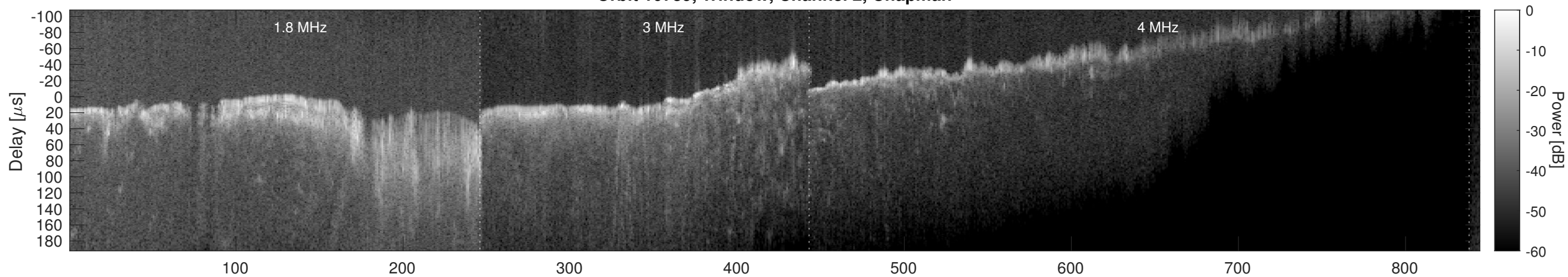
Orbit 10739, Window, Channel 2, Optimized
