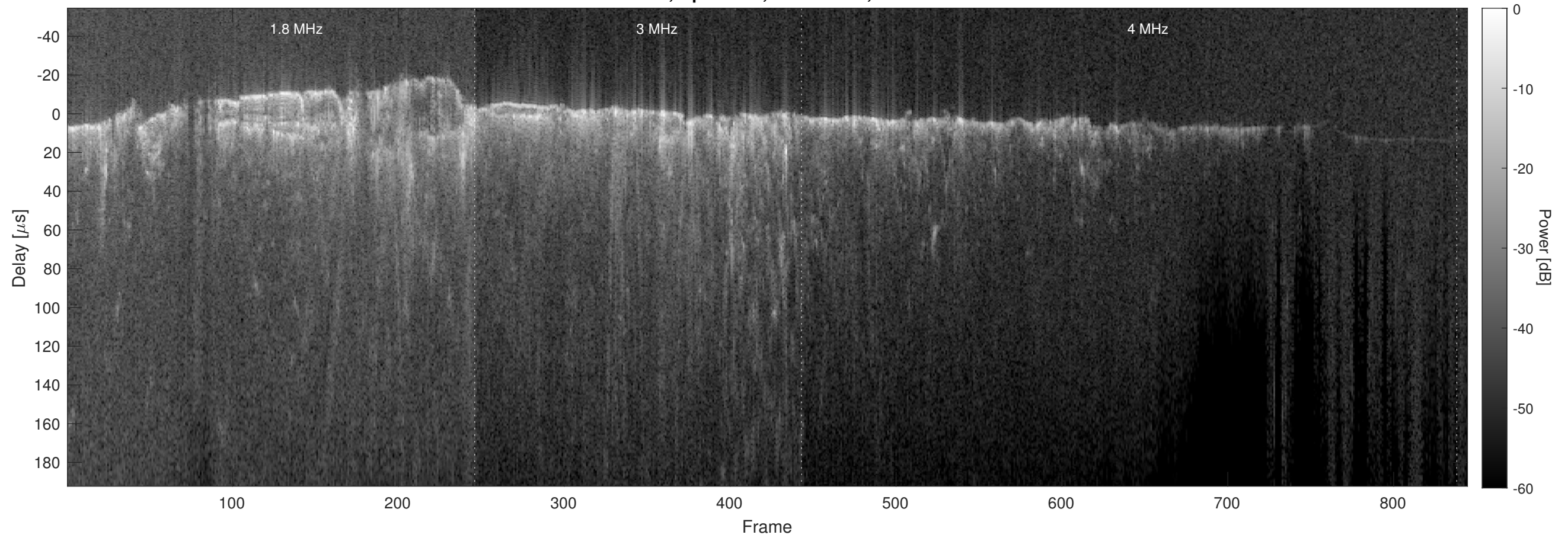
Orbit 10739, Optimized, No Window, Channel 2
