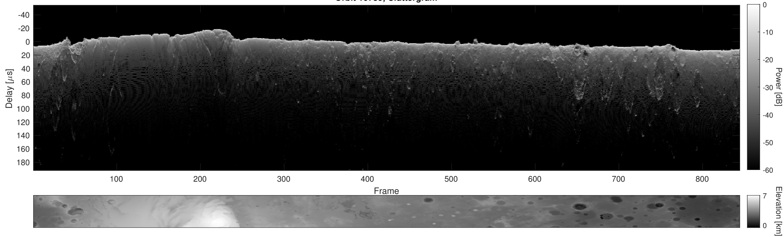
Orbit 10739, Cluttergram
