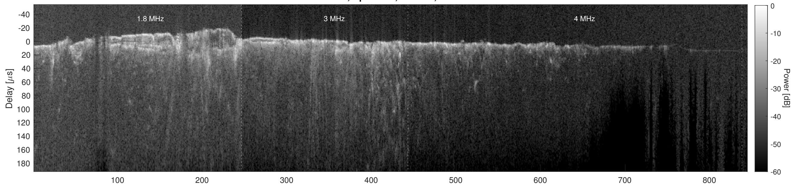
Orbit 10739, Cluttergram
