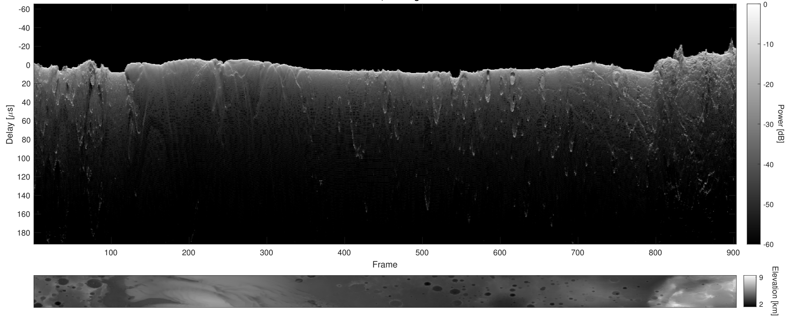
Orbit 10740, Cluttergram
