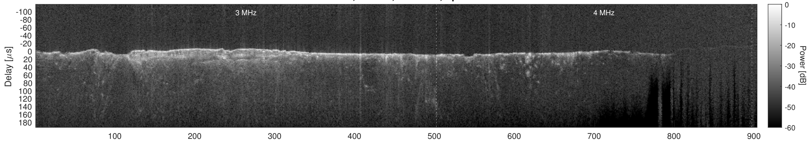
Orbit 10740, Cluttergram
