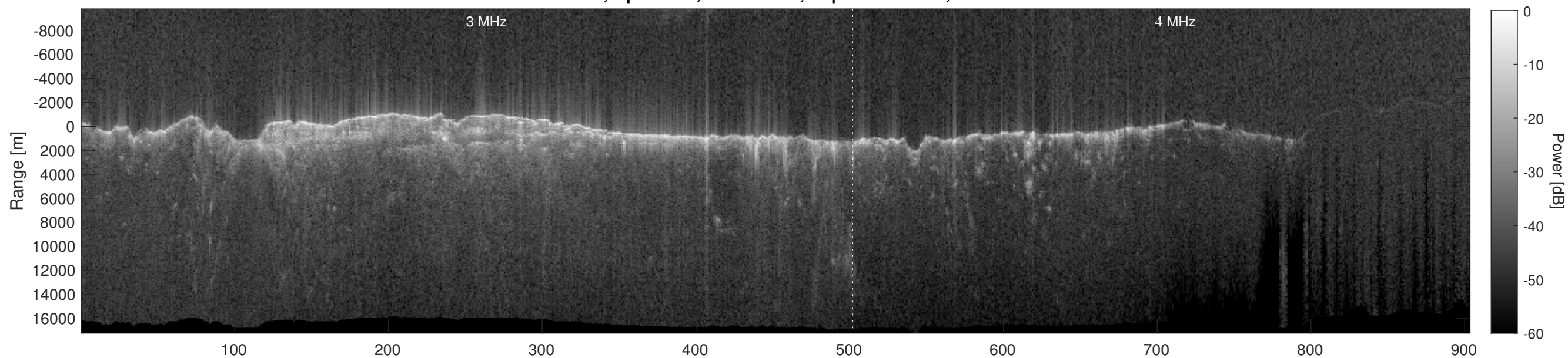
Orbit 10740, Depth-Corrected Cluttergram
