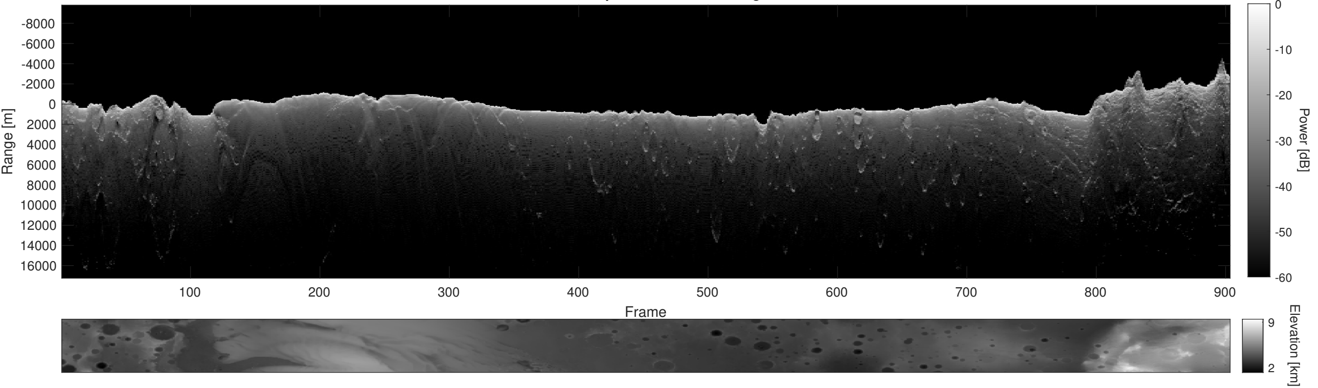
Orbit 10740, Depth-Corrected Cluttergram
