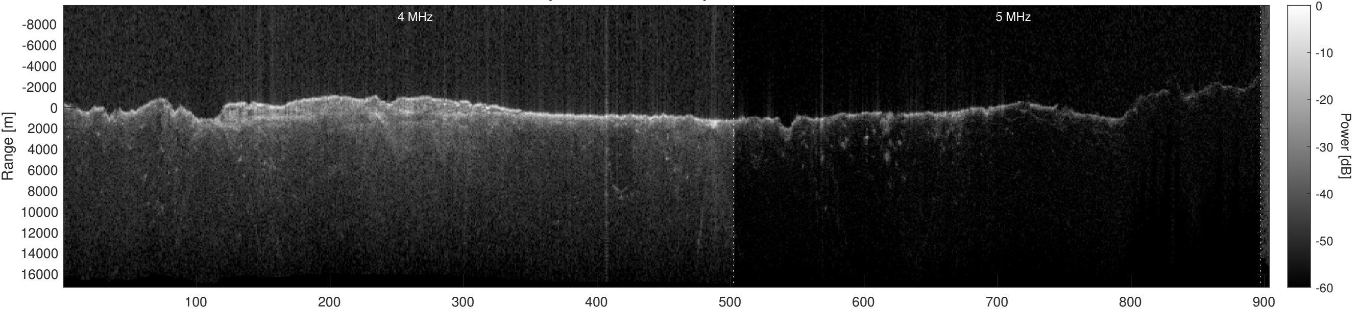
Orbit 10740, Optimized, Window, Depth-Corrected, Channel 2
