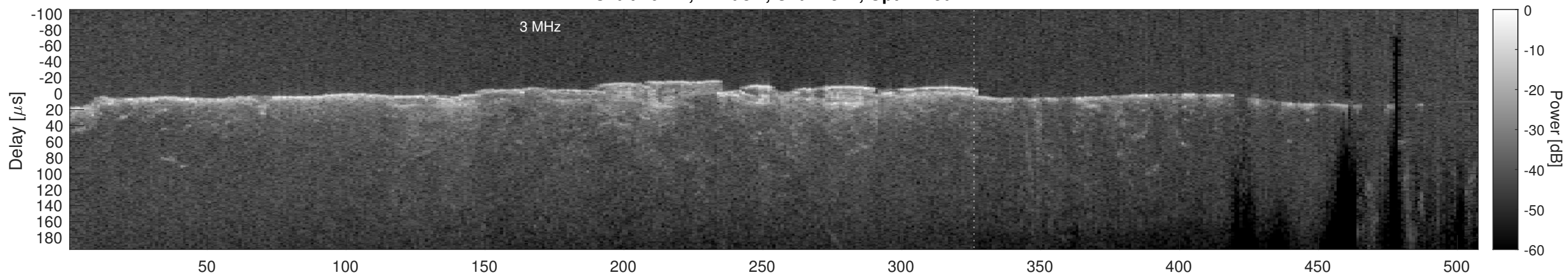
Orbit 10741, Cluttergram
