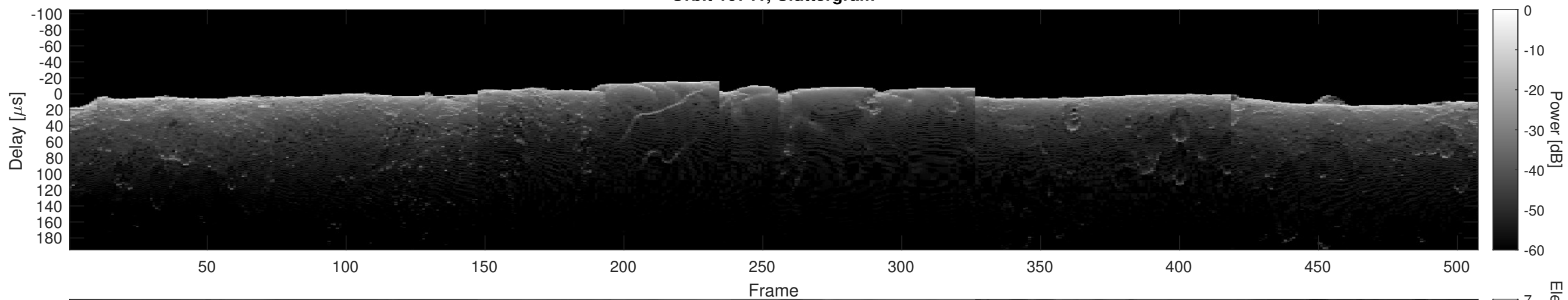
Orbit 10741, Cluttergram
