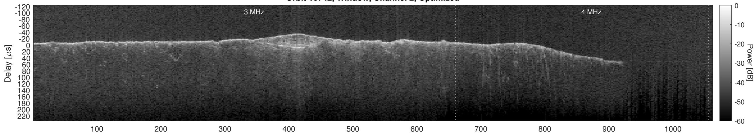
Orbit 10742, Cluttergram
