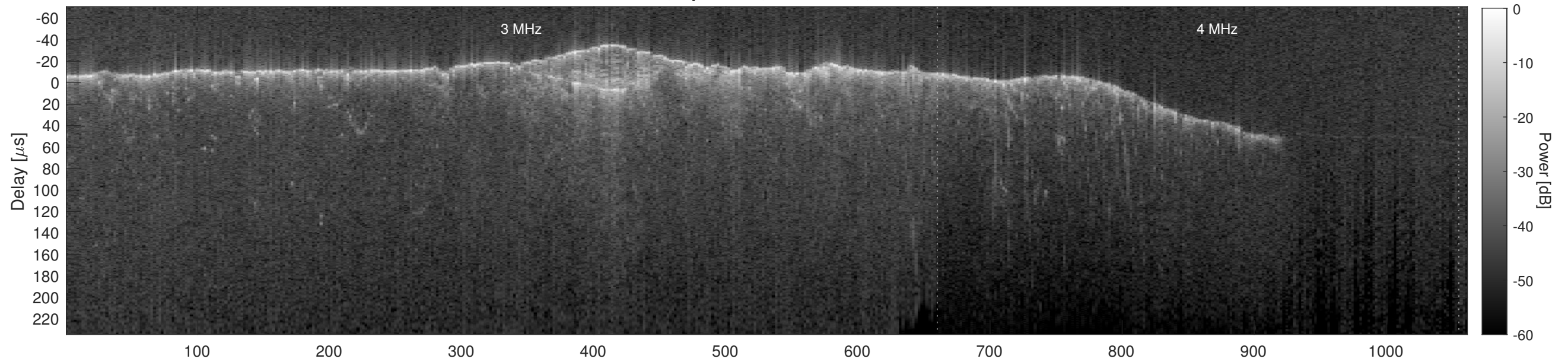
Orbit 10742, Cluttergram
