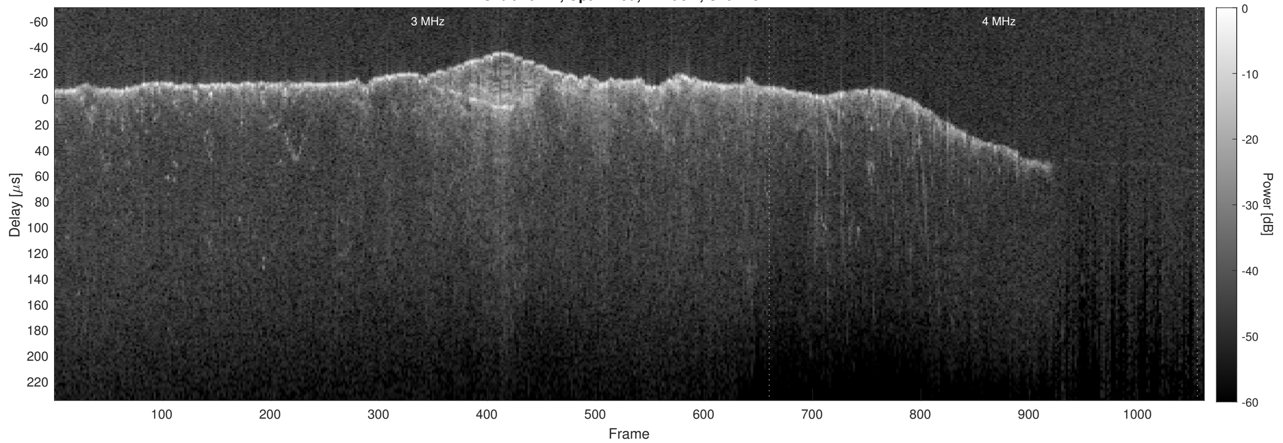
Orbit 10742, Optimized, Window, Channel 2
