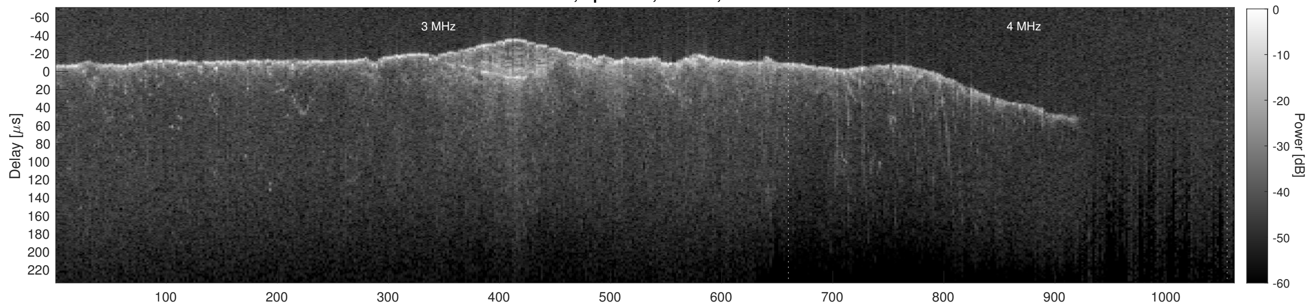
Orbit 10742, Cluttergram
