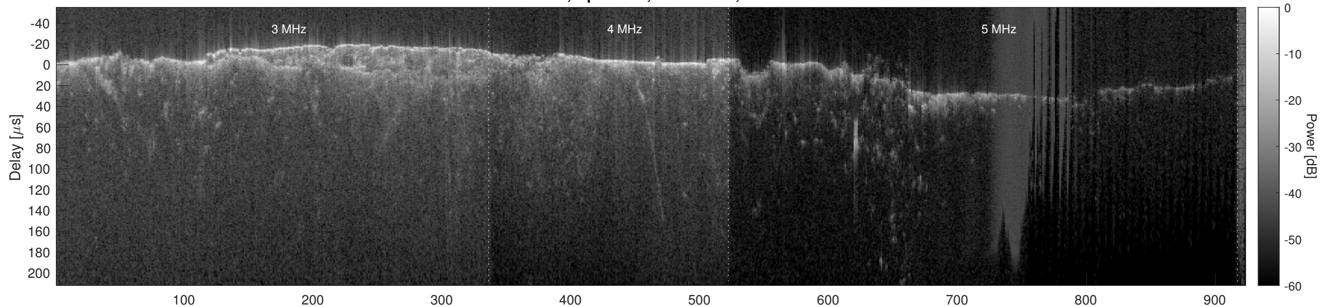
Orbit 10743, Optimized, No Window, Channel 2
