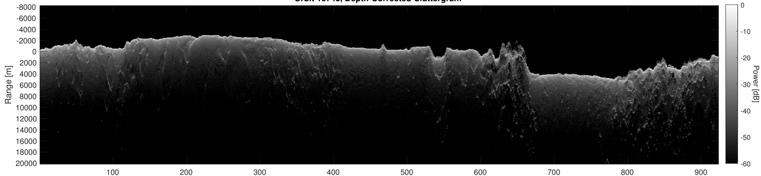
Orbit 10743, Depth-Corrected Cluttergram
