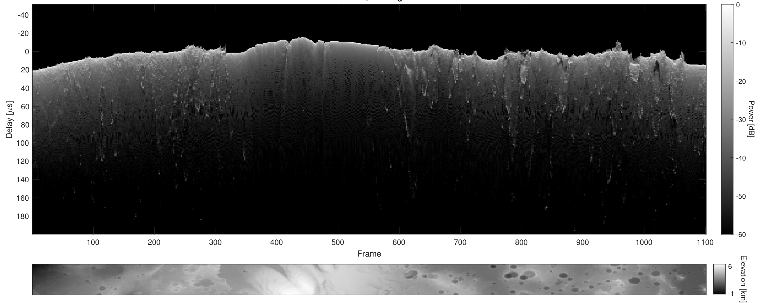
Orbit 10744, Cluttergram
