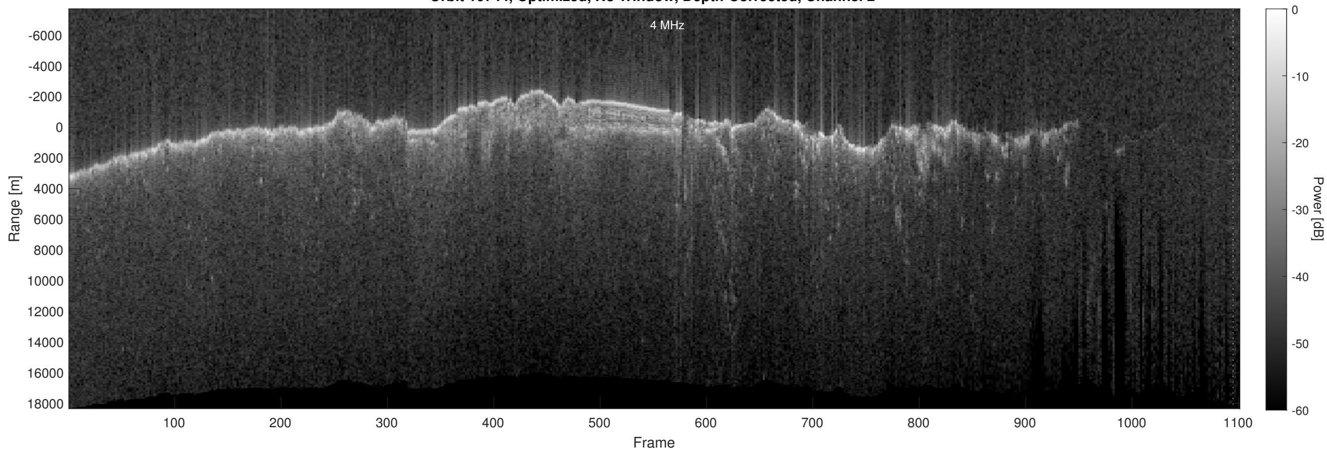
Orbit 10744, Optimized, No Window, Depth-Corrected, Channel 2
