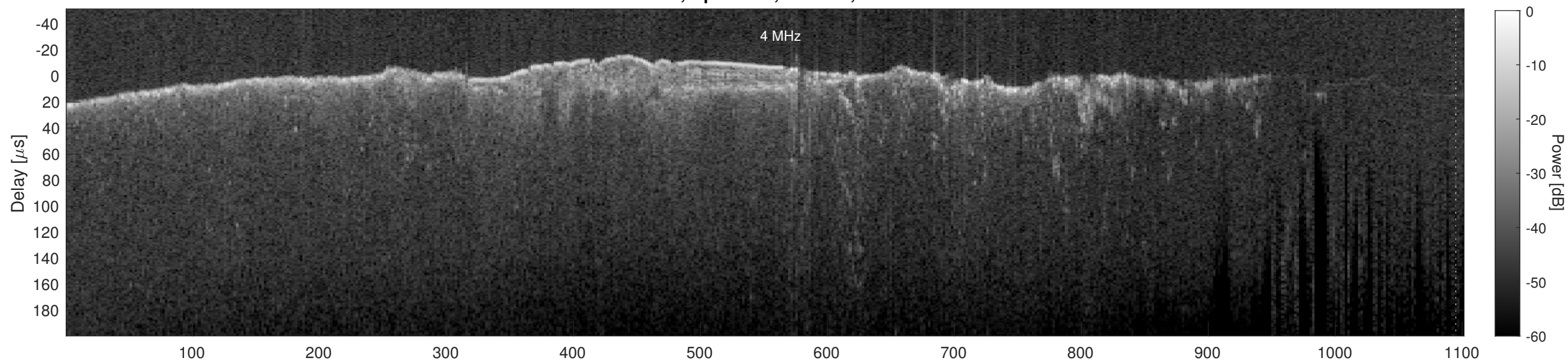
Orbit 10744, Cluttergram
