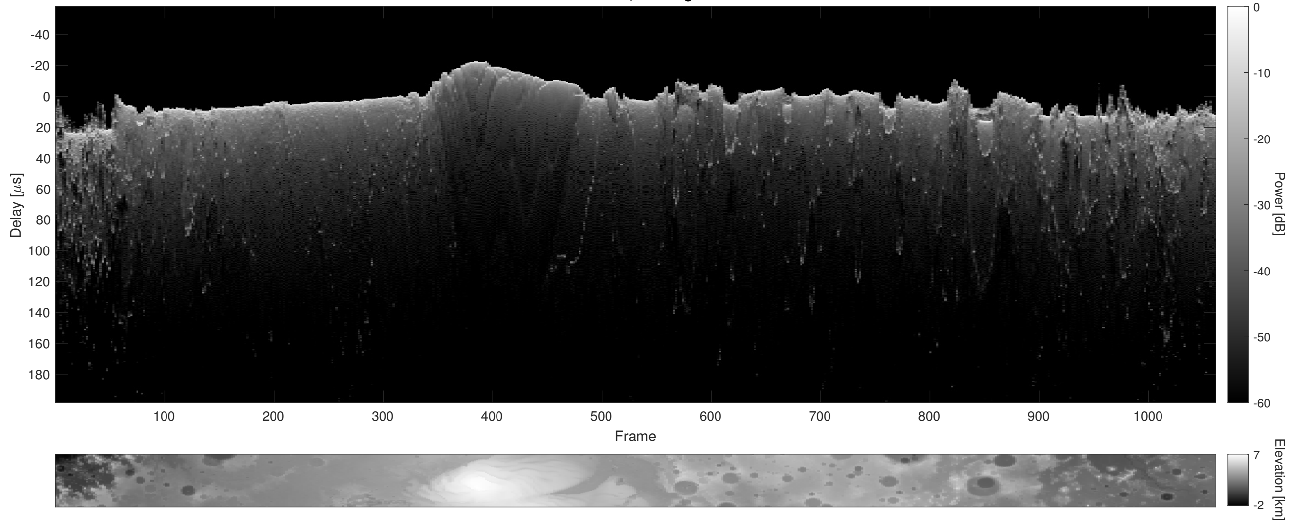
Orbit 10745, Cluttergram
