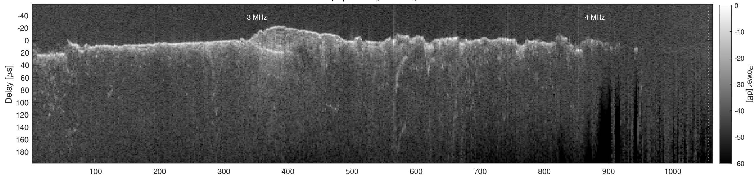
Orbit 10745, Cluttergram
