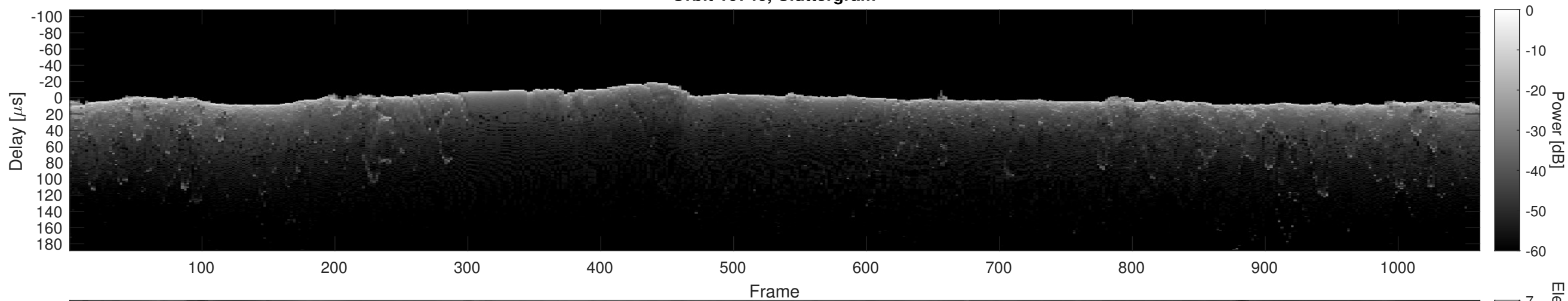
Orbit 10746, Cluttergram
