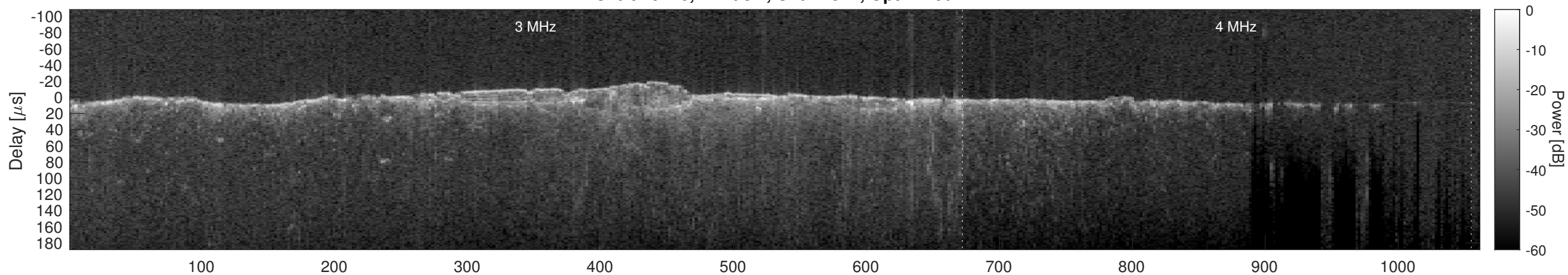
Orbit 10746, Cluttergram
