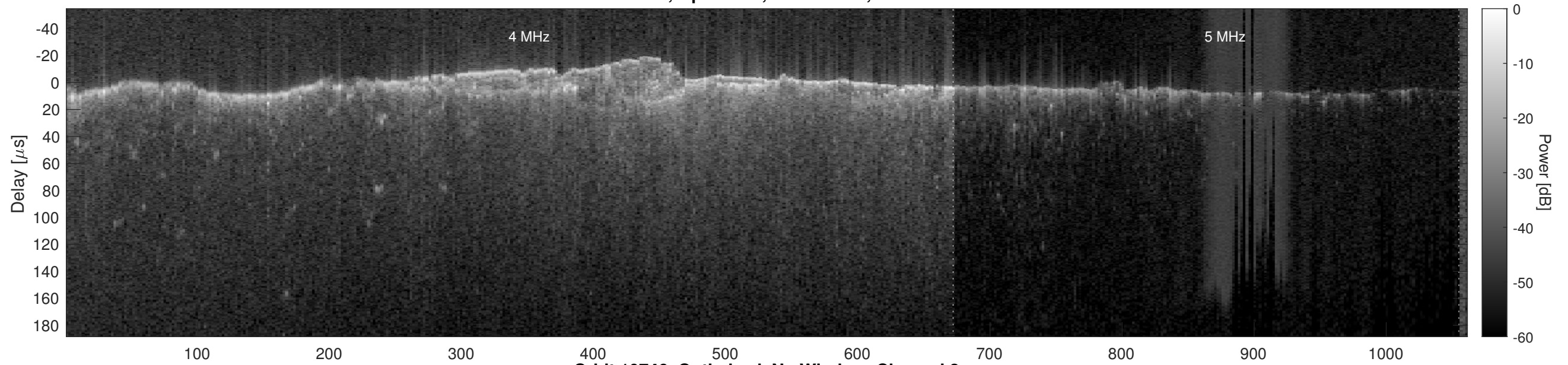
Orbit 10746, Optimized, No Window, Channel 2
