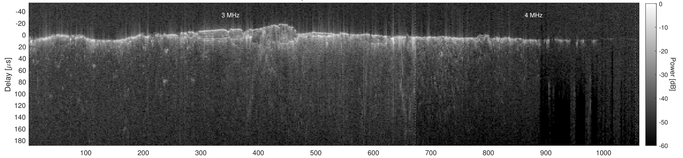
Orbit 10746, Cluttergram
