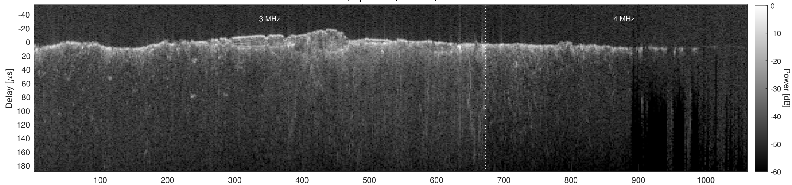
Orbit 10746, Cluttergram
