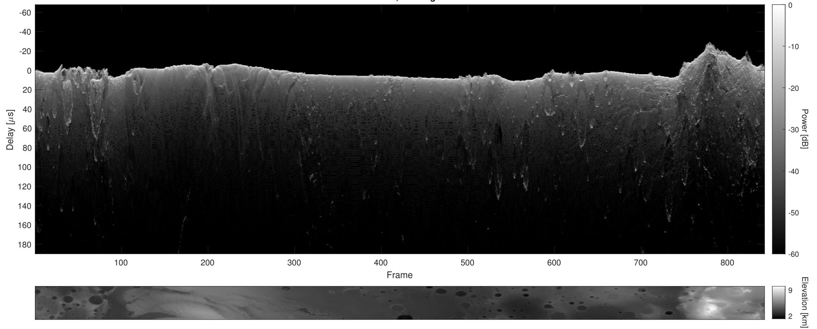
Orbit 10747, Cluttergram
