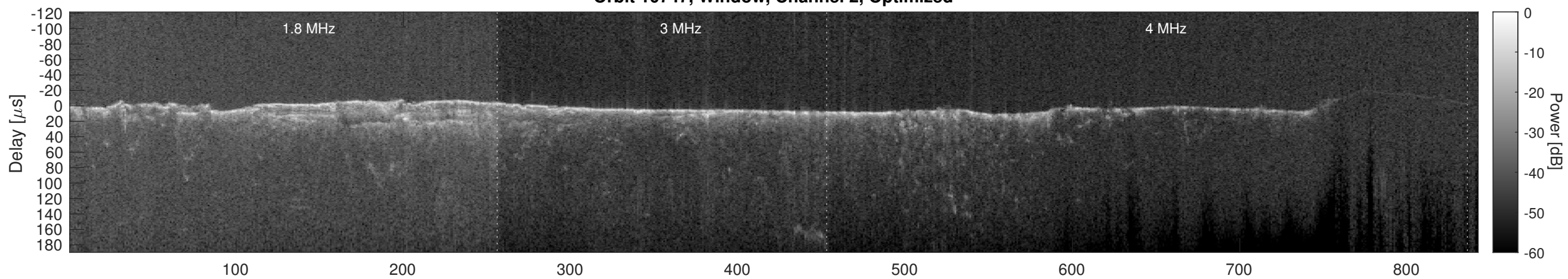
Orbit 10747, Cluttergram
