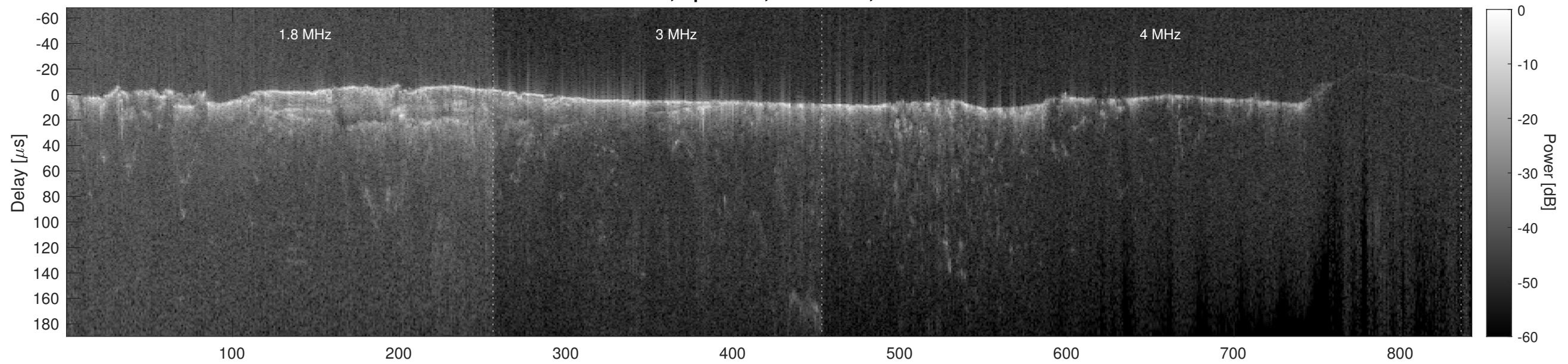
Orbit 10747, Cluttergram
