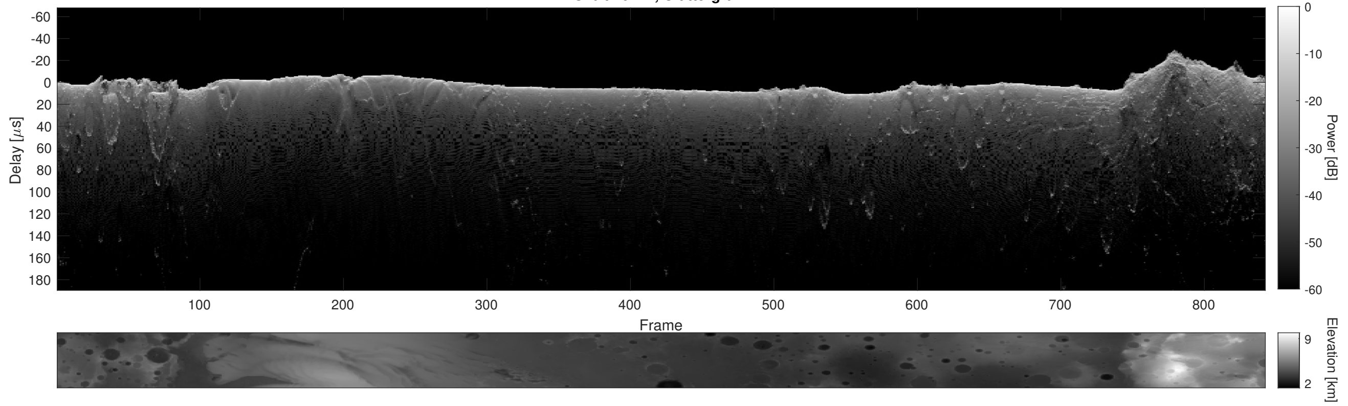
Orbit 10747, Cluttergram
