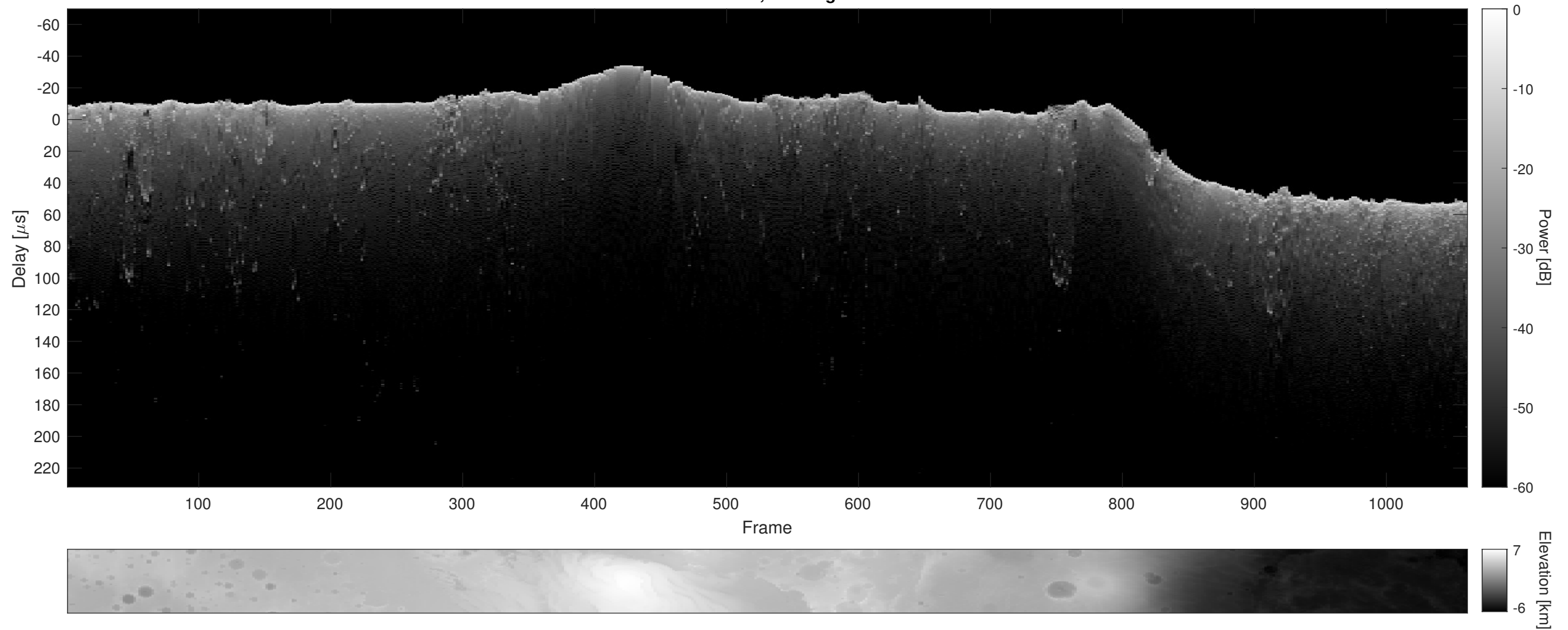
Orbit 10749, Cluttergram
