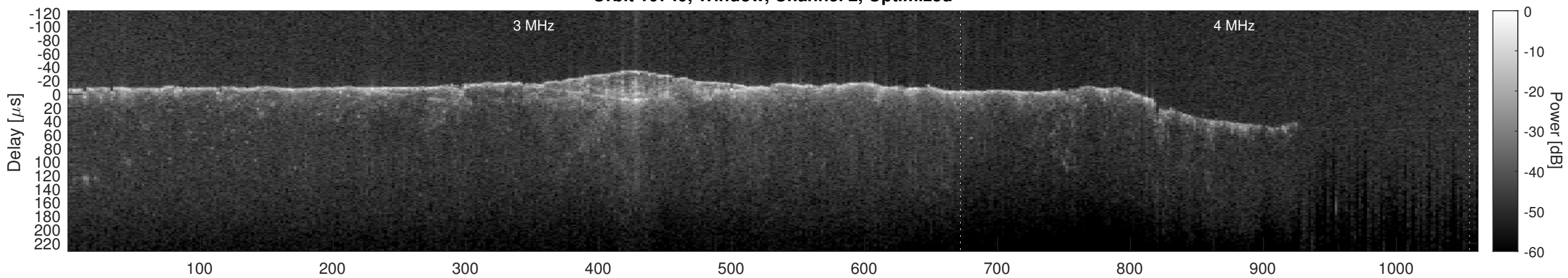
Orbit 10749, Cluttergram
