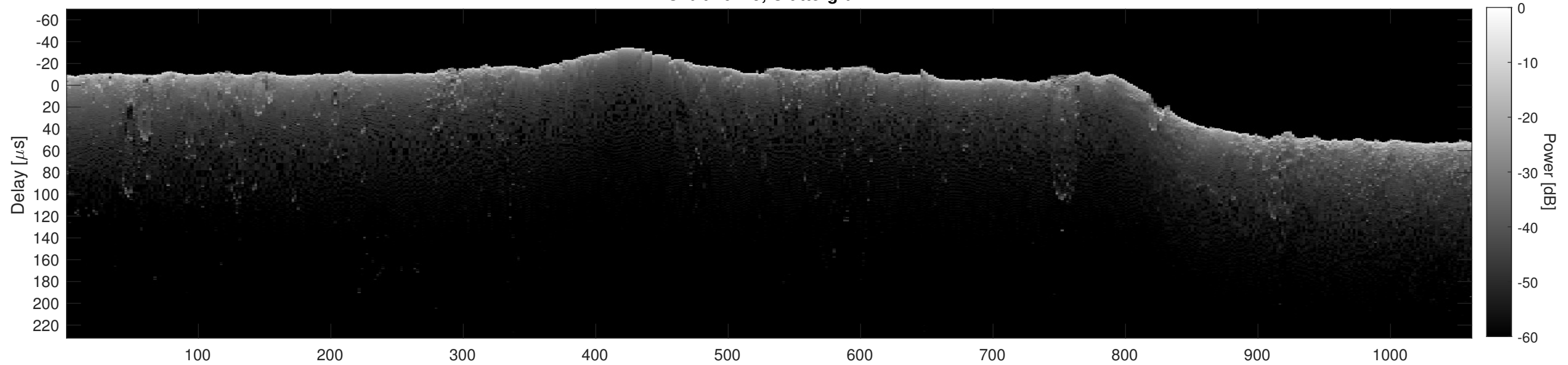
Orbit 10749, Cluttergram
