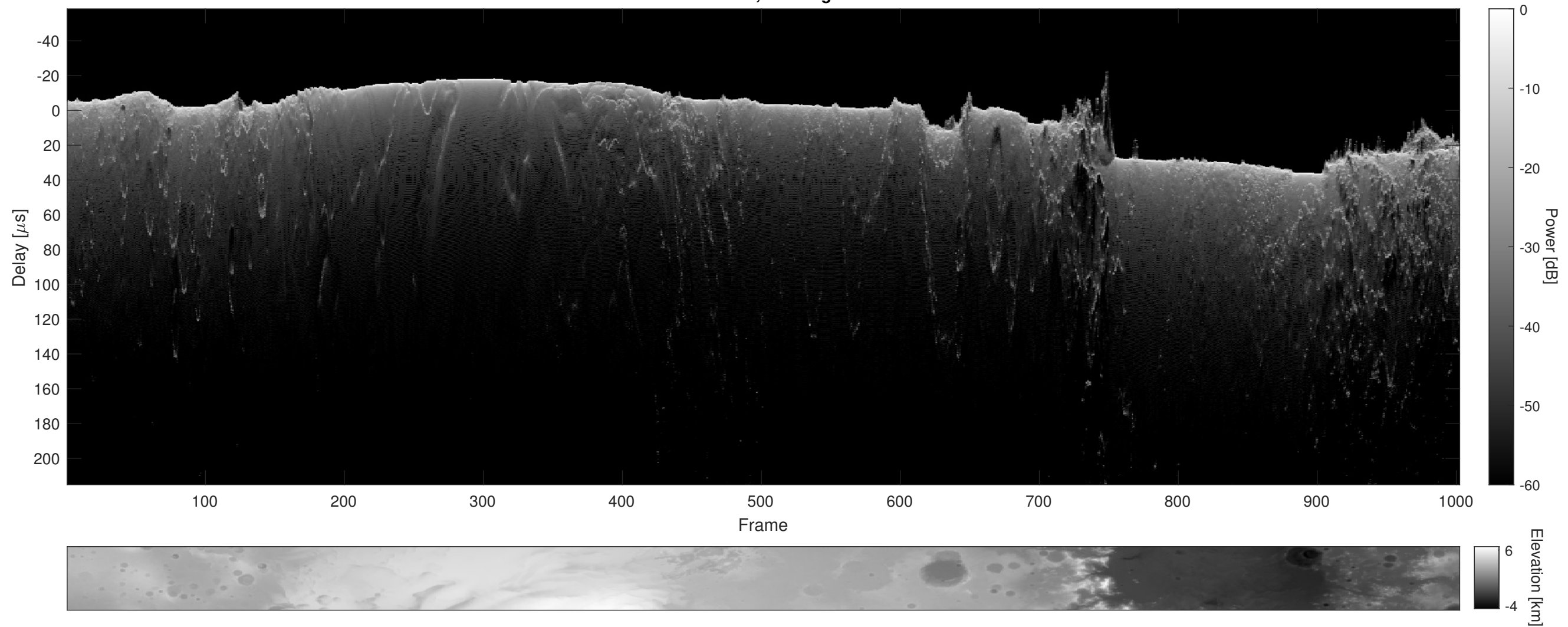
Orbit 10750, Cluttergram
