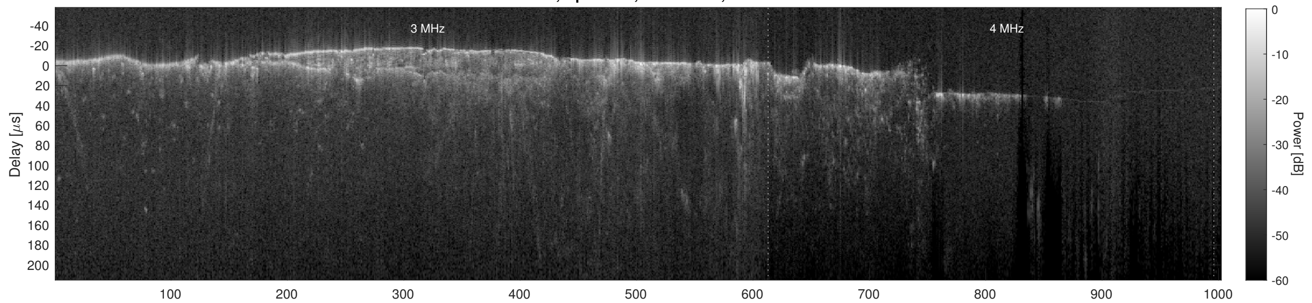
Orbit 10750, Cluttergram
