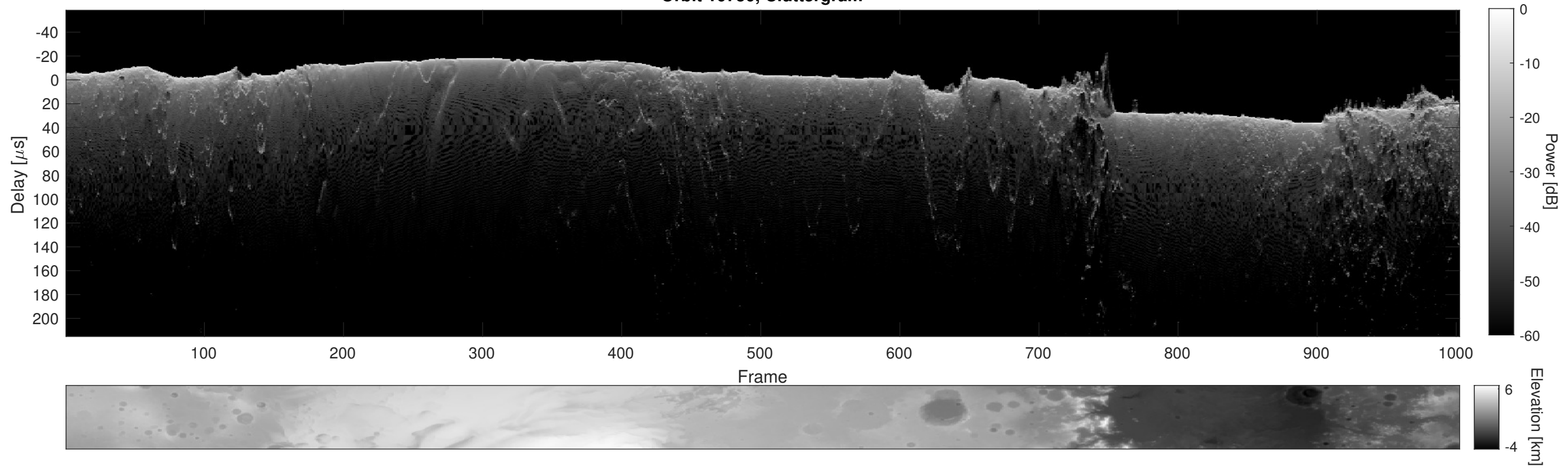
Orbit 10750, Cluttergram
