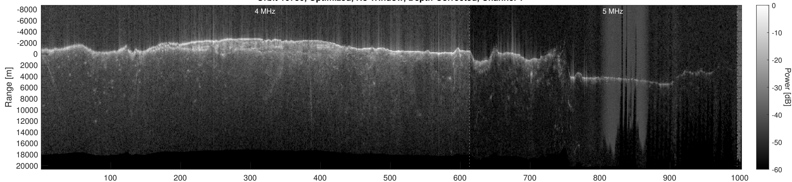
Orbit 10750, Optimized, No Window, Depth-Corrected, Channel 2
