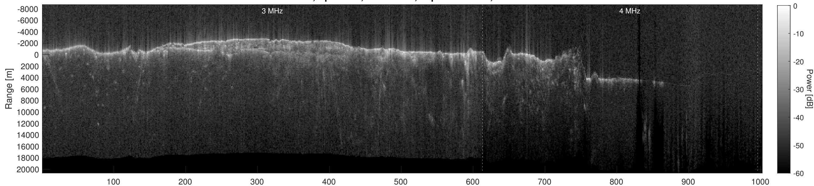
Orbit 10750, Depth-Corrected Cluttergram
