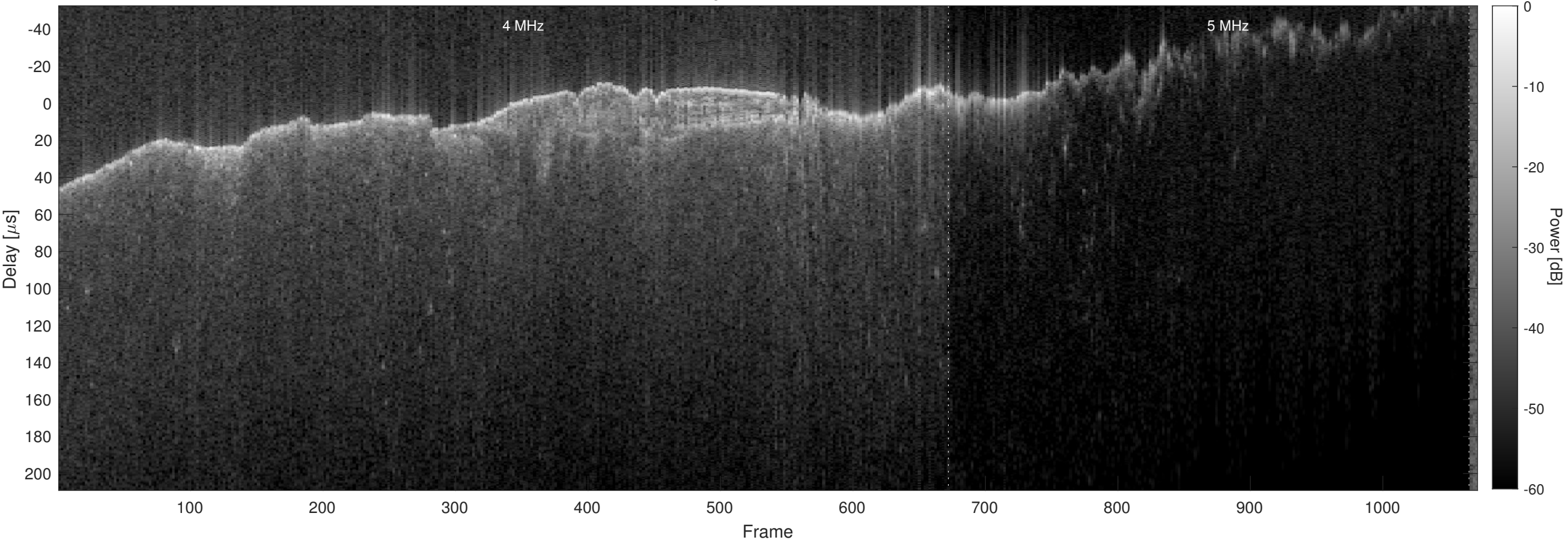
Orbit 10751, Chapman, No Window, Channel 2
