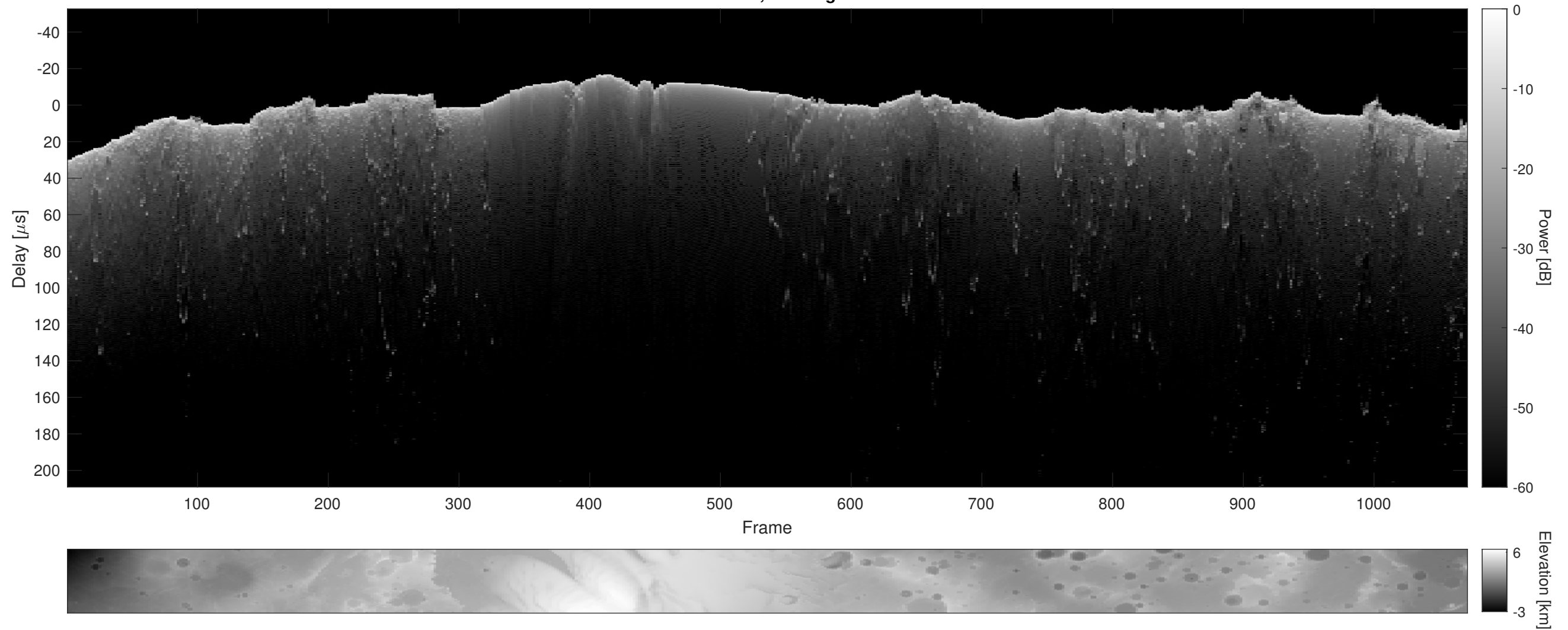
Orbit 10751, Cluttergram
