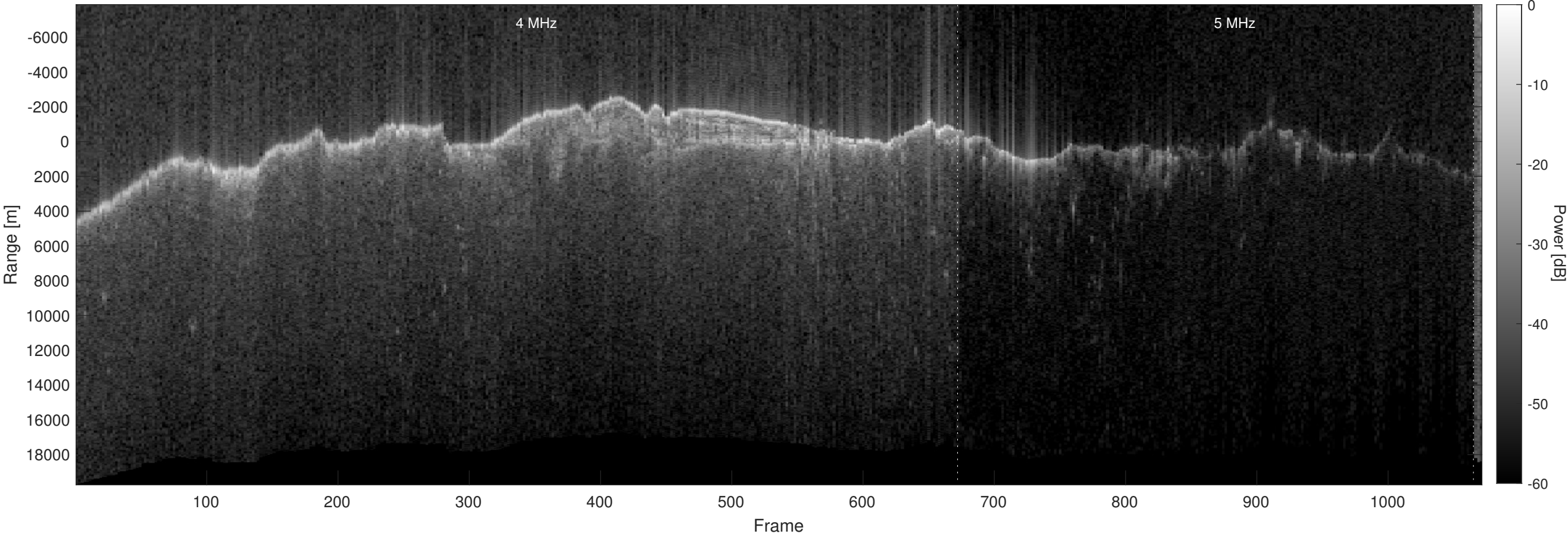
Orbit 10751, Optimized, No Window, Depth-Corrected, Channel 2
